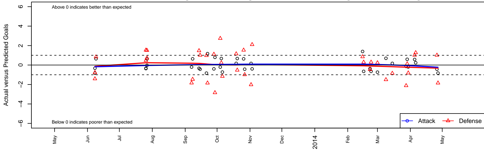
BSC Portland Black G99 Dots are actual minus expected GF (blue circles) and GA (red triangles). Blue line is smoothed change in attack strength. Red is smoothed change in defense strength.
